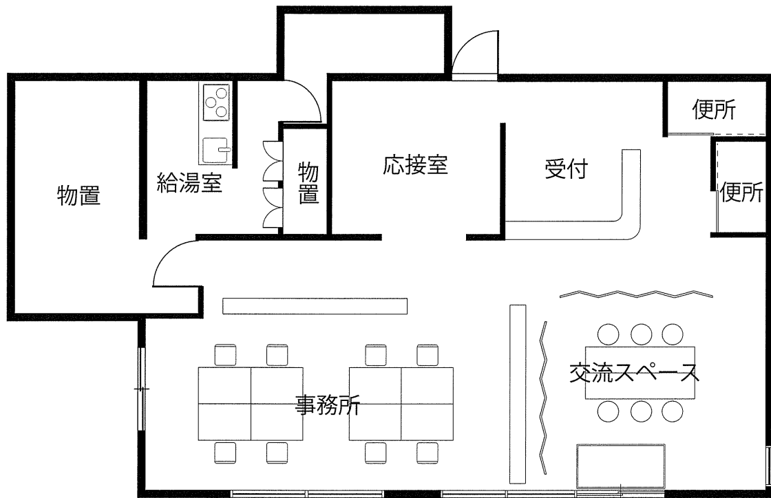
1 F PLAN 1/100
