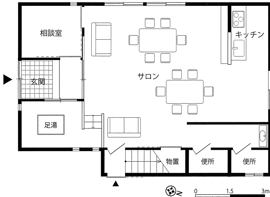
1 F PLAN 1/100
