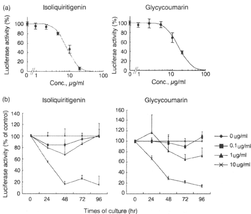
Figure 3 Dose- and time-dependent suppression of HCV replication by isoliquiritigenin and glycycomarin. (a) Relative log (dose)-response plots for isoliquiritigenin or glycycomarin. Error bars indicate mean \pm SD of triplicate analyses. Calculated probit curves are overlaid in each plot. (b) Huh7/Rep-Feo cells were cultured with the concentrations of isoliquiritigenin and glycycomarin indicated. The internal luciferase activities were measured at times of culture indicated. Assays were performed in triplicate. Error bars indicate mean \pm SD.
