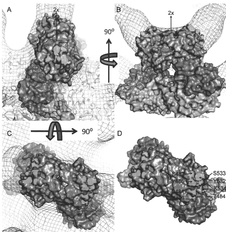
FIG. 3. The binding site of Fab224 antibody. (A) The cryo-EM density map of VLP-Fab224 was fitted with the crystal structure of PORF2 and viewed along a bound Fab molecule. One PORF2 dimer is presented as a solid surface and colored light magenta for the S domain, blue violet for the M domain, and dark gray for the P domain. The neighboring dimers are drawn in ribbon mode and colored wheat. (B) Side view of a PORF2 dimer fitted into the cryo-EM density map. (C) A PORF2 dimer viewed along the 2-fold axis and overlapped with the cryo-EM density map. (D) Top view of a PORF2 dimer viewed along the 2-fold axis. The amino acids in PORF2 responsible for binding to Fab224 are labeled. The PORF2 dimer is presented as a solid surface and colored in gray, violet, and light magenta for the P domain, the M domain, and the S domain, respectively. The residues along the Fab binding interface are colored according to the element, with green for carbon, blue for nitrogen, and red for oxygen.
