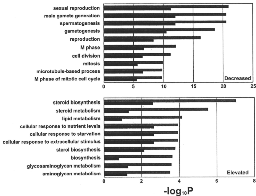
Figure 2. Comparison of Ten Top-ranked Gene Ontology (GO) Categories Significantly Over-Represented in the Two Subsets (1,709 Decreased, Upper Panel; 903 Elevated, Lower Panel) of NOA-related Target Genes
