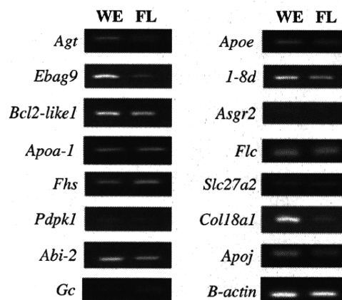
Fig. 2 Expression of candidate erythroid genes in developing mouse embryos. RT-PCR analyses of candidate genes in mouse embryos. We used RT-PCR to examine the expression patterns of the mouse homologues of each candidate gene in 10.5 dpc whole embryos (WE) and 12.5 dpc FL in ICR mouse embryos
