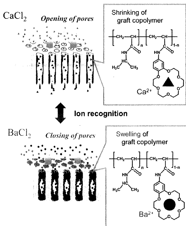
Fig. 1. Concept of a molecular recognition ion gating membrane made of porous PE-g-NIPAM-co-BCAm.
