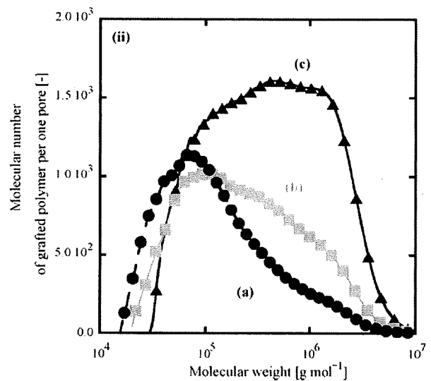
Fig. 9. GPC measurement of samples of grafted NIPAM polymer using various filling ratios: (a) 9%, (b) 21%, and (c) 58%; (i) GPC chromatograph, and (ii) molecular number of grafted NIPAM polymers per one pore.
