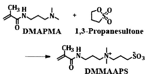
Scheme 1. Synthesis scheme of non-detergent sulfobetaine monomer, N,N -dimethyl (methacrylamidopropyl) ammonium propanesulfonate (DMMAAPS).
