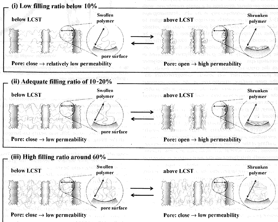
Fig. 12. Schematic illustration of the pore gating of a thermal-responsive gating membrane; (i) the low filling ratio below 10%, (ii) the adequate filling ratio of 10–20%, and (iii) the high filling ratio around 60%.
