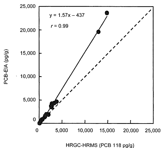
Figure 4. Comparison of PCB-EIA concentrations with HRGC-HRMS measurements of PCB 118 concentrations in fish samples ( n = 20 ). The dashed line represents x = y .
