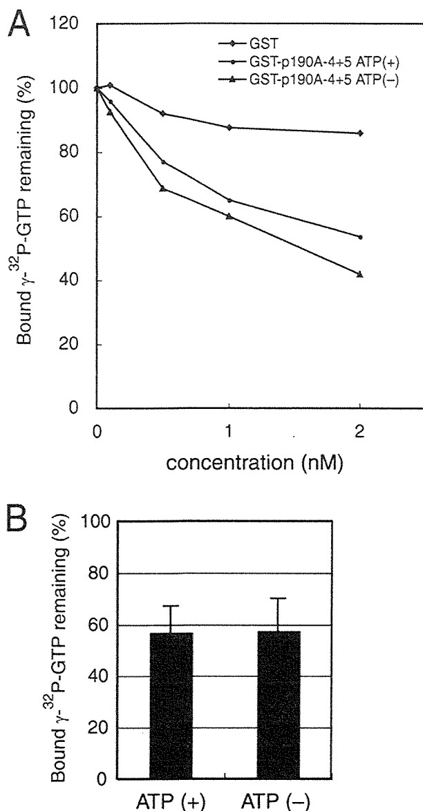
FIGURE 4. Effect of phosphorylation of p190A RhoGAP by Rho-kinase on its GAP activity in vitro . A, GST-p190A RhoGAP-4+5 was produced in Sf9 cells with a baculovirus system and purified on glutathione-Sepharose beads. Hydrolysis of GTP-bound GST-RhoA was monitored with GST (squares), non-phosphorylated GST-p190A RhoGAP-4+5 (triangles), or phosphorylated GST-p190A RhoGAP-4+5 (circles) for 5 min at 30 °C. The result is representative of three independent experiments. B, 1 \mu M [ \gamma - ^{32} P]GTP-bound GST-RhoA was incubated with 1 nM nonphosphorylated RhoGAP-4+5 or phosphorylated GST-p190A RhoGAP-4+5 for 5 min at 30 °C. Data are indicated as mean \pm S.D. ( n = 20, respectively, p = 0.82).
