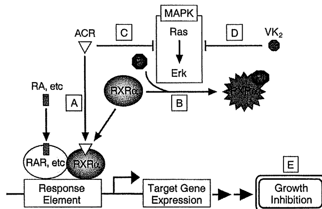
Fig. 6. Schematic representation of the effect of vitamin K 2 (VK 2 ) and acyclic retinoid (ACR) on retinoid X receptor (RXR) \alpha phosphorylation in hepatocellular carcinoma cells. (a) In normal hepatocytes, ACR binds to RXR \alpha and transactivates downstream genes via retinoid X receptor responsive element (RXRE), which may regulate cell proliferation. (b) In hepatocellular carcinoma (HCC) cells, the Ras/mitogen-activated protein kinase (MAPK) pathway is highly activated and phosphorylates RXR \alpha at serine residues, thus impairing the functions of the receptor. (c) ACR and (d) VK 2 cooperatively suppress the Ras/MAPK signaling pathway, inhibit phosphorylation of RXR \alpha , restore the function of the receptor, and thus subsequently activate the transcriptional activity of the responsive element, including RXRE. (e) These effects may contribute to growth inhibition of the hepatoma cells.
