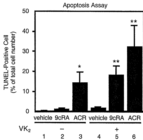
Fig. 3. Effects of the combination of retinoids plus vitamin K 2 (VK 2 ) on the induction of apoptosis in HuH7 cells. The cells were treated for 48 h with vehicle (column 1), 1.0 μM 9- cis -retinoic acid (9cRA) (column 2), 1.0 μM acyclic retinoid (ACR) (column 3), 10 μM VK 2 (column 4), the combination of 10 μM VK 2 plus 1.0 μM 9cRA (column 5), or the combination of 10 μM VK 2 plus 1.0 μM ACR (column 6). The cells were then stained using a terminal deoxynucleotidyl transferase-mediated dUTP nick-end labeling (TUNEL) method, and TUNEL-positive cells were counted and expressed as a percentage of total cell numbers (500 cells were counted in each flask). Values are the mean ± SD (n = 5). Asterisks represent significant difference (P < 0.05) compared to column 1. Representative results from three independent experiments with similar results are shown.
