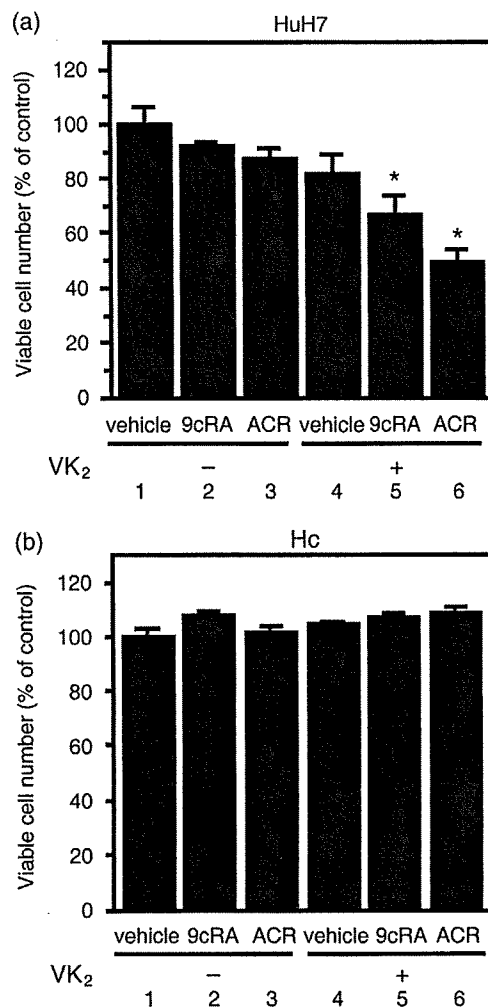
Fig. 1. Effect of retinoids and vitamin K 2 (VK 2 ) on the proliferation of (a) HuH7 human hepatocellular carcinoma cells and (b) Hc human normal hepatocytes. HuH7 cells and Hc cells were cultured for 72 h in the presence of vehicle (column 1), 10 μM 9- cis -retinoic acid (9cRA) (column 2), 5 μM acyclic retinoid (ACR) (column 3), 10 μM VK 2 (column 4), the combination of 10 μM VK 2 plus 10 μM 9cRA (column 5), or the combination of 10 μM VK 2 plus 5 μM ACR (column 6). Cell number was determined using the Trypan Blue dye exclusion method and expressed as a percentage vehicle. Values are the mean ± SD ( n = 5). An asterisk represents significant differences ( P < 0.01) compared to vehicle (column 1). Similar results were obtained in a repeat experiment.
