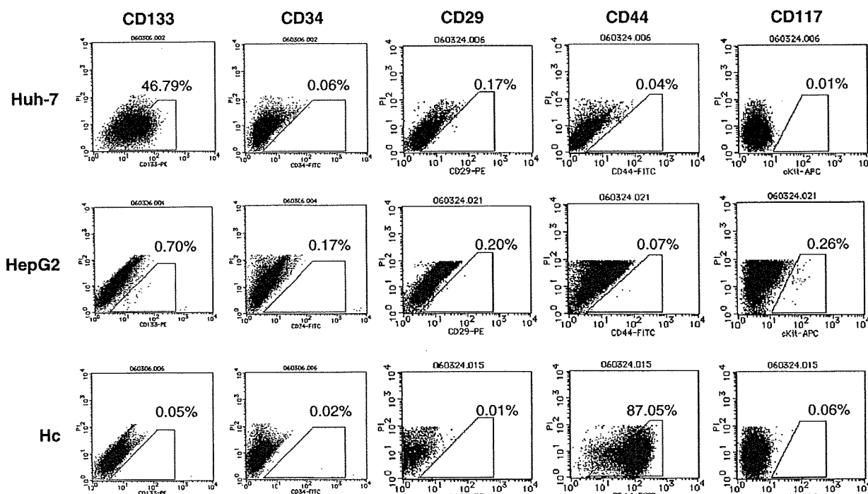
Fig. 1. The expression of cell surface markers was examined by FACS analysis. Huh-7, HepG2, and Hc cells were stained with fluorescence-conjugated anti-CD133, CD34, CD29, CD44, and CD117. The results shown are representative of at least five independent experiments.
