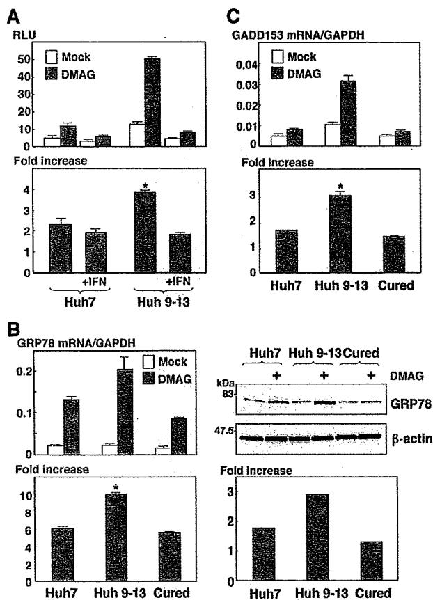
FIG. 6. Effect of Hsp90 inhibitor on the induction of the UPR in HCV replicon cells. (A) Huh7 and Huh9-13 replicon cells were transfected with a reporter plasmid, pGRP78-luc, and an internal-control plasmid, pRL-TK. The transfected cells were treated with IFN- \alpha (+IFN) from 6 to 36 h posttransfection or left untreated and then further incubated for 6 h in the presence or absence of 1 \mu M DMAG. The resulting cells were harvested and subjected to a dual-luciferase assay. The firefly luciferase activity is indicated as the RLU (top) after standardization with that of Renilla luciferase. The enhancement of promoter activity by treatment with DMAG is presented as the increase (bottom). (B) Huh7 cells, Huh9-13 cells, and Huh9-13 cells cured by IFN- \alpha treatment (Cured) were cultured for 6 h in the presence or absence of 1 \mu M DMAG, and the amount of GRP78 mRNA was measured by real-time PCR. The value of the mRNA was normalized with the amount of GAPDH mRNA (upper left), and the transcriptional enhancement by treatment with DMAG is presented as the increase (lower left). The expression levels of GRP78 and \beta -actin in the cells were determined by immunoblotting (upper right) and are presented as the increase (lower right). (C) The amounts of GADD153 mRNA in Huh7 cells, Huh9-13 cells, and the cured cells cultured for 6 h in the presence or absence of 1 \mu M DMAG were measured by real-time PCR. The values of the mRNA were normalized with the amount of GAPDH mRNA (top), and the transcriptional enhancement by treatment with DMAG is presented as the increase (bottom). The error bars indicate standard deviations. The asterisks indicate significant differences ( P < 0.01 ) versus the control value. The data shown are representative of three independent experiments.
