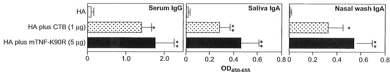
Fig. 5. mTNF-K90R induced mucosal IgA and IgG responses against influenza virus HA in mice. BALB/c mice were immunized intranasally with HA together with 1 µg CTB or 5 µg mTNF-K90R. One week after the last immunization, HA-specific IgG in serum at a 1:500 dilution and IgA in nasal or saliva at a 1:8 dilution were assessed by ELISA at a 1:8 dilution. Data represents the mean of absorbance 450 nm (reference wavelength, 655 nm). N.D.; not detected. Data are presented as means \pm SEM ( n = 4-6 ; * P < 0.05 , ** P < 0.01 versus value for HA alone treated group by ANOVA).
