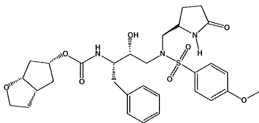
FIG. 1. Structure of GRL-02031.
