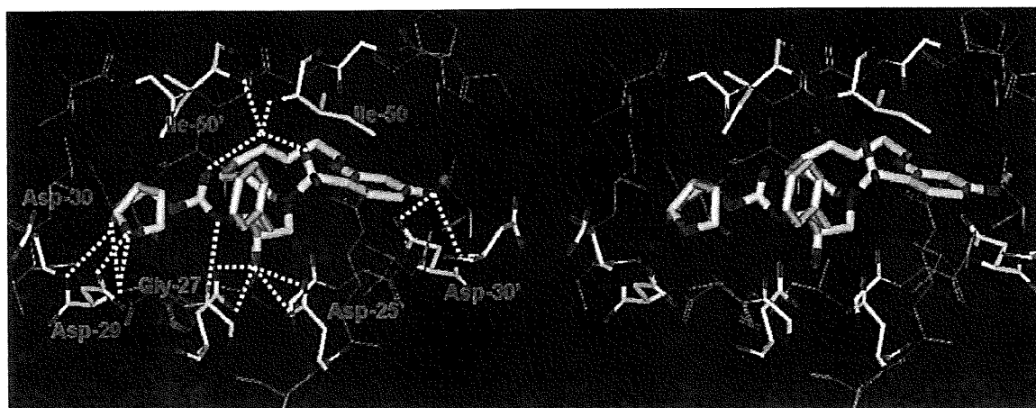
Figure 3. A stereoview of the X-ray structure of macrocyclic inhibitor 14c (light gray)-bound HIV-1 protease. All strong hydrogen bonding interactions are shown as dotted lines.
