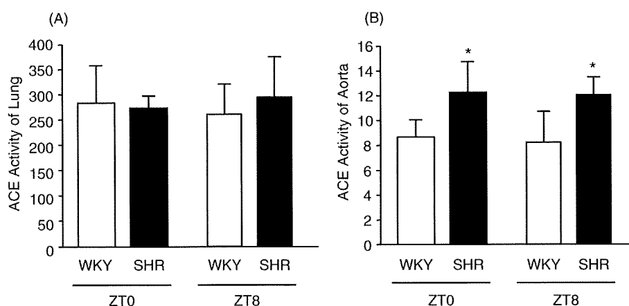
Figure 3. Angiotensin converting enzyme (ACE) activity of lung (A) and aorta (B) at ZT0 and ZT8 in the SHR (solid bar) and WKY rats (open bar). Values reported as nmol/mg wet weight/hour. Data represent the mean \pm SEM for six independent experiments in the SHR and WKY rats. * p < 0.05 vs. WKY rats.
