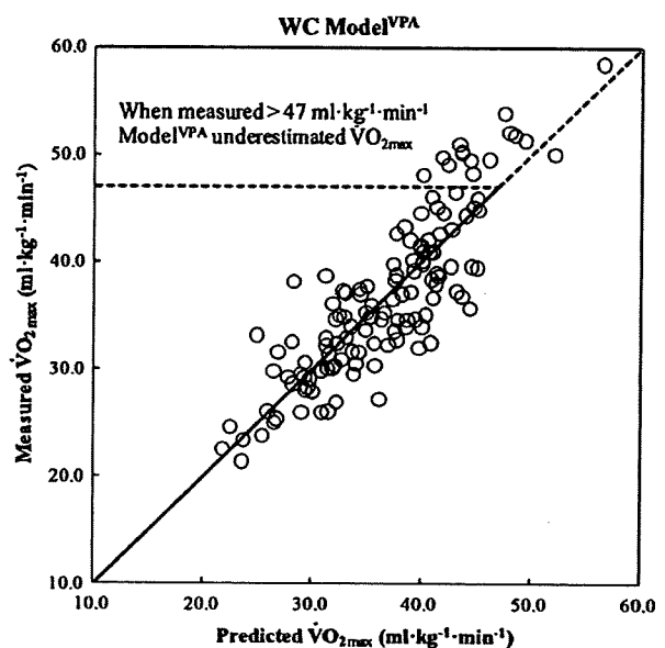
Fig. 2 Relationships between the measured and predicted \dot{V}O_{2max} values for the multiple regression model VPA in the entire sample ( n = 127 ). The solid line is the line of equality (measured \dot{V}O_{2max} = predicted \dot{V}O_{2max} ). The areas within the dashed lines show where the model VPA tends to underestimate \dot{V}O_{2max}
