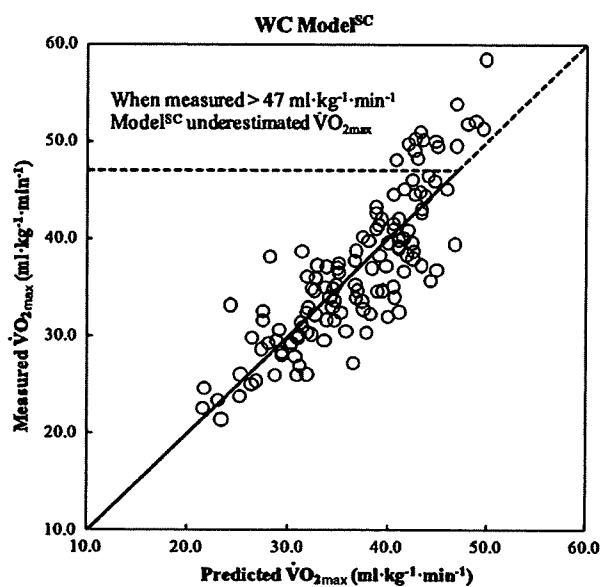
Fig. 1 Relationships between the measured and predicted \dot{V}O_{2max} values for the multiple regression model SC in the entire sample ( n = 127 ). The solid line is the line of equality (measured \dot{V}O_{2max} = predicted \dot{V}O_{2max} ). The areas within the dashed lines show where the model SC tends to underestimate \dot{V}O_{2max}
