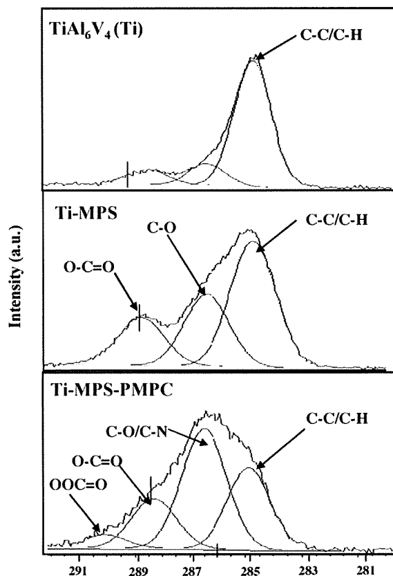
Fig. 2. XPS high resolution ( \text{C}1\text{s} ) spectra of the modified and unmodified \text{TiAl}_6\text{V}_4 samples.
