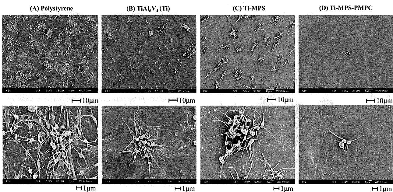
Fig. 5. SEM micrographs of polystyrene, unmodified and modified TiAl_6V_4 samples after contact with ovine blood (heparin 6U/mL) for 2.5 h at 37 °C. (A) polystyrene (B) Ti (C) Ti-MPS (D) Ti-MPS-PMPC.
