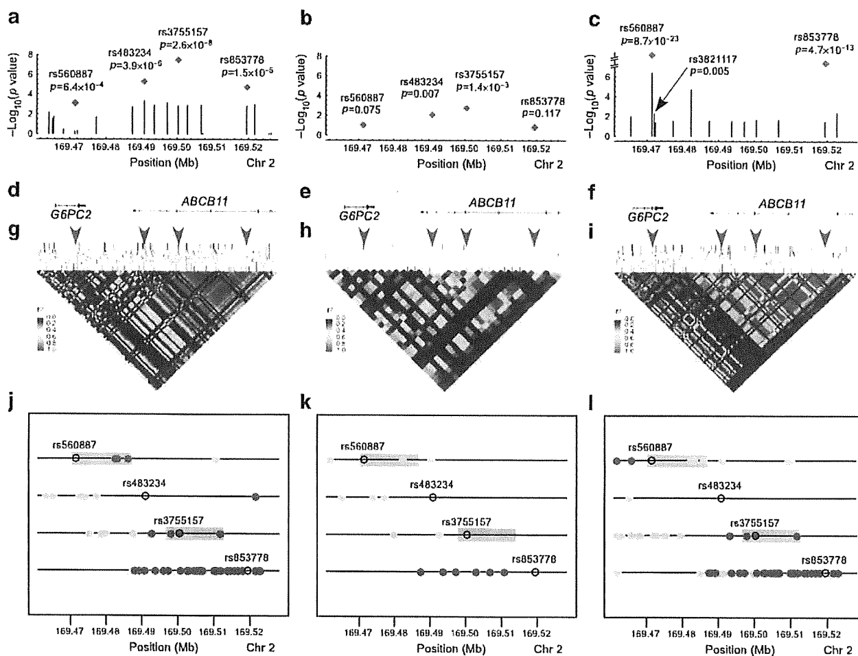
Fig. 1 Plots of FPG association, and LD and SNP partitioning for the G6PC2-ABCB11 region in Japanese (a, d, g, j), Sri Lankan (b, e, h, k) and Europeans (c, f, i, l). Association results for Europeans are drawn from the published studies [14, 17]. a–c Bar graphs of all genotyped SNPs that passed the quality control (ESM Table 6) in the Japanese GWA scan (a) and those in the published European GWA scan [14] (c) with -\log_{10}(p \text{ value}) for FPG plotted against chromosome position in Mb. Red diamonds, p values for the genotypes of general populations ( n=4,813 in Japanese, n=2,319 in Sri Lankan) and meta-analysis data ( >12,000 in the ENGAGE consortium [17]). d–f Genomic location of G6PC2 and ABCB11 genes with intron and
