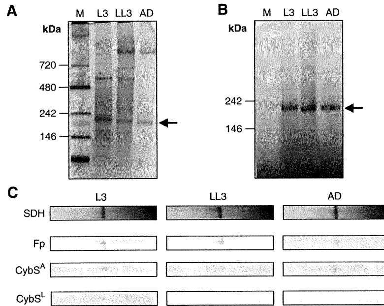
Fig. 4. BN-PAGE analysis. BN-PAGE analysis of mitochondria from A. suum L3 larvae, LL3 larvae and adults (1.5 \mu\text{mol}/\text{min} SDH activity). (A) CBB-stain. Arrow indicates expected SDH active bands. (B) SDH activity stained in gels of Native PAGE™ Bis-Tris gel (4–16%). Arrow shows SDH active bands. (C) Western blotting after SDS-PAGE, following BN-PAGE. Antibodies used were the same as in Fig. 3. The size marker is Native Mark Unstained Protein Standard (Invitrogen).
