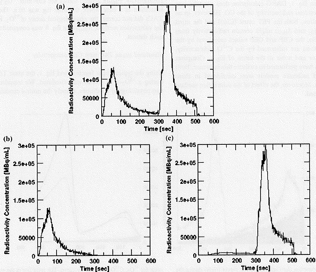
Fig. 3 Separation of the input function for the ^{15}O_2-C^{15}O_2 scan. Total input function (a), ^{15}O_2 input function (b), and C^{15}O_2 input function (c) separated from the total input function. The radioactivity observed earlier than 300 s in the graph (c) is the recirculation water
