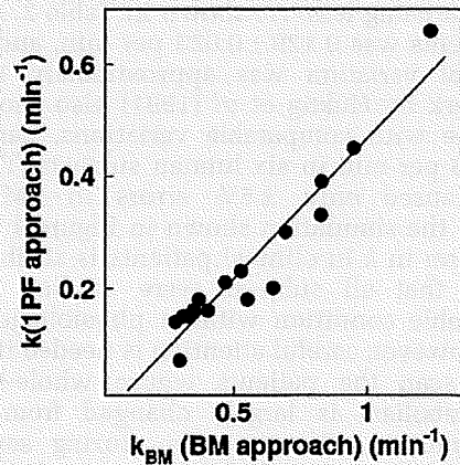
Figure 4 Comparison of the production rates of RW obtained by BM approach and those by 1PF approach in five monkeys at various anesthetic and PaCO 2 levels. The regression line was y = 0.50x - 0.034 (per min) ( r = 0.95 ).
