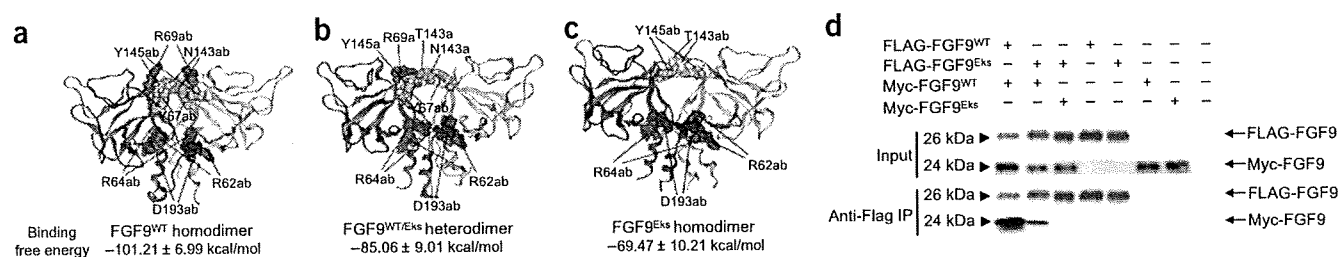
Figure 8 FGF9 WT modulates FGF9 Eks action by forming FGF9 WT -FGF9 Eks heterodimers. (a–c) Proposed solution structures for FGF9 WT homodimer (a), FGF9 WT/Eks heterodimer (b) and FGF9 Eks homodimer (c). Amino acid residues contributing to hydrogen bond formation involved in dimerization are drawn in ball-and-stick and space-filling modes. The single-letter amino acid code, residue number and chain code are indicated for each of these residues. Computed binding free energy of each dimer is shown under the respective illustrated structure. Data are represented as mean \pm s.d. of energies obtained from 200 molecular-dynamics snapshots in respective molecular-dynamics trajectory. (d) FGF9 WT is capable of forming dimers with FGF9 Eks . The expression of FGF9 WT homodimers, FGF9 WT/Eks heterodimers and FGF9 Eks homodimers was analyzed using immunoprecipitation and protein blots. The expression vectors for FLAG- or Myc-tagged FGF9 WT and FGF9 Eks were transfected into COS7 cells and culture supernatants were subjected to immunoprecipitation and protein blot analysis. (e–h) Less severe elbow joint synostosis in Fgf9 Eks/+ than Fgf9 Eks/- . Forelimbs from Fgf9 +/- , Fgf9 Eks/+ , Fgf9 Eks/- and Fgf9 Eks/Eks embryos at E17.5 were stained with Alcian blue and Alizarin red. Synostotic change is restricted to the cartilaginous component in Fgf9 Eks/+ embryos, whereas it is extended to the bony component in Fgf9 Eks/- and Fgf9 Eks/Eks embryos. h, humerus; r, radius; u, ulna.
