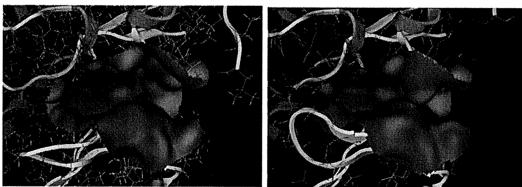
Figure 4. Binding pockets in two different X-ray crystal structures for CDK2. The left figure indicates the binding pocket in the CDK2-Oxindole inhibitor complex (PDB Id: 1FVV). This structure was used in our study. The right figure indicates the binding pocket in the CDK2-NU2058 inhibitor complex (PDB Id: 1H1P). The hydrophobic regions in the binding pocket are drawn in blue, and the hydrophilic regions are drawn in red. From this figure, it is clear that large hydrophobic regions were located in both binding pockets. In contrast, the shapes of the two binding pockets were considerably different, which means that the binding pocket of CDK2 was flexible. doi:10.1371/journal.pcbi.1000528.g004
