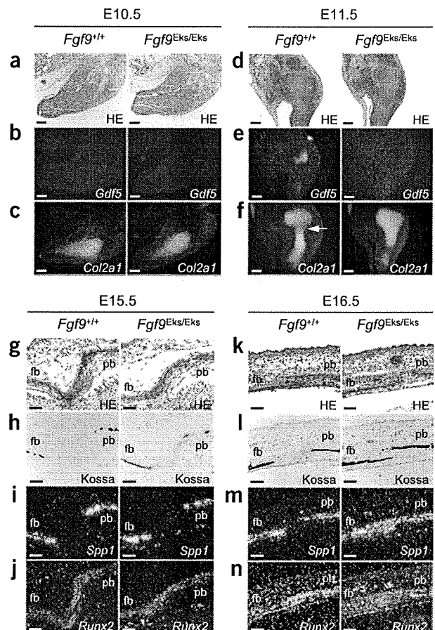
Figure 2 Synostotic phenotypes in Fgf9 Eks / Eks mice. (a–f) Defects in early specification of prospective elbow joints in Fgf9 Eks / Eks embryos. Hematoxylin and eosin staining (a,d) and in situ detection of Gdf5 (b,e) and Col2a1 (c,f) in the forelimb buds of Fgf9 +/+ and Fgf9 Eks / Eks embryos at E10.5 and E11.5. In Fgf9 +/+ embryos, there was Gdf5 expression at the prospective elbow joint (e, left), which was demarcated as the gap of Col2a1 expression (f, arrow), at E11.5. In Fgf9 Eks / Eks embryos, there was not Gdf5 expression at the prospective elbow joint (e, right). Scale bars, 100 μm. (g–n) Ectopic osteogenesis at the coronal sutures in Fgf9 Eks / Eks fetuses. Hematoxylin and eosin staining (g,k) and von Kossa staining (h,l) and in situ detection of Spp1 (i,m) and Runx2 (j,n) in the coronal suture of Fgf9 +/+ and Fgf9 Eks / Eks fetuses at E15.5 and E16.5. Note the ectopic ossification in the suture of Fgf9 Eks / Eks at E16.5. fb, frontal bone; pb, parietal bone. Scale bars, 100 μm.
