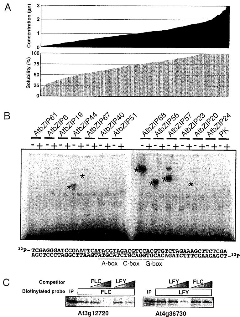
Fig. 1. Construction of a Protein Library of Arabidopsis Transcription Factors and Its Application to DNA Binding Assay.
