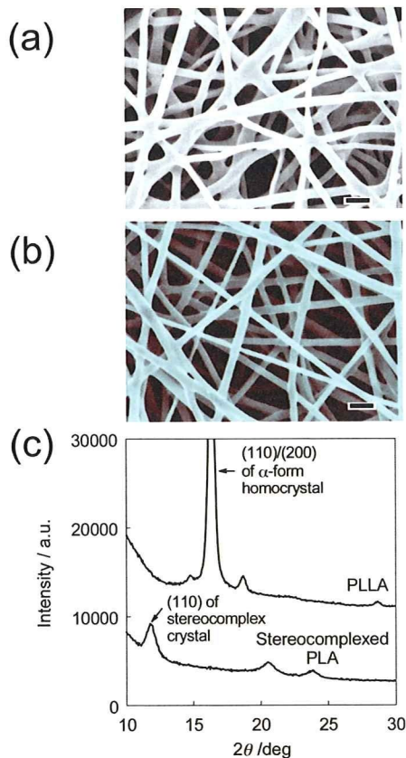
Figure 1. SEM images of (a) PLLA and (b) stereocomplexed PLA nanofibers and (c) wide-angle X-ray diffraction patterns of PLLA and stereocomplexed PLA nanofibers. Scale bars = 1 \mu\text{m} . PLLA nanofiber shows diffraction peaks at 2\theta = 15.1, 16.5 (assigned to (110)/(200)), and 18.1^\circ that are assigned to \alpha -form homocrystal of PLA. On the other hand, stereocomplexed PLA nanofiber showed diffraction peaks at 2\theta = 12.0 (assigned to (110)), 20.8 , and 24.1^\circ that are assigned only to stereocomplex crystal of PLA.
