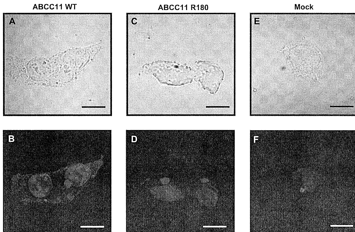
Figure 3. Immunocytochemical staining of Flp-In-293 cells expressing ABCC11 WT and R180 variant proteins. Differential interference (A, C, E) and immunofluorescence images (B, D, F). ABCC11 proteins were immunologically detected with ABCC11-specific polyclonal antibody and Alexa Fluor 488 (green). Cellular nuclei were stained by propidium iodide (red). Antibody interacts with epitope peptide residing in cytoplasmic domain (aa 746–804) between TM6 and TM7. Since Gly180 or Arg180 residue resides in TMI, this amino acid alteration (Gly180Arg) does not affect immunoreactivity. Scale bars = 10 \mu m.
