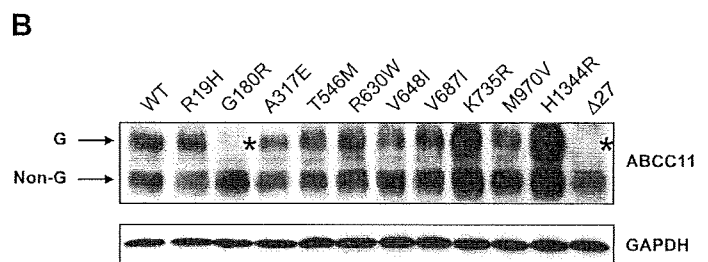
Figure 6. Effect of nonsynonymous SNPs and a \Delta 27 mutation on the N -linked glycosylation status of ABCC11. A ) Locations of hitherto reported nonsynonymous SNPs and \Delta 27 are indicated in putative structure of ABCC11. B ) Variants of nonsynonymous SNPs and \Delta 27 were created by site-directed mutagenesis with PCR primers listed in Supplemental Table 3. Those variant forms were expressed in Flp-In-293 cells. N -linked glycosylated (G) and nonglycosylated (non-G) forms of ABCC11 protein were detected by immunoblotting. Asterisk (*) indicates no N -linked glycosylation of ABCC11. C ) Levels of ABCC11 WT and \Delta 27 mutant proteins in Flp-In-293 cells. Samples were processed in the same manner as described in Fig. 4A. D ) Effect of MG132 on expression levels of ABCC11 WT and \Delta 27 mutant proteins. ABCC11 and GAPDH (loading marker) were detected by immunoblotting. Data are expressed as means \pm SD; n = 3 .
