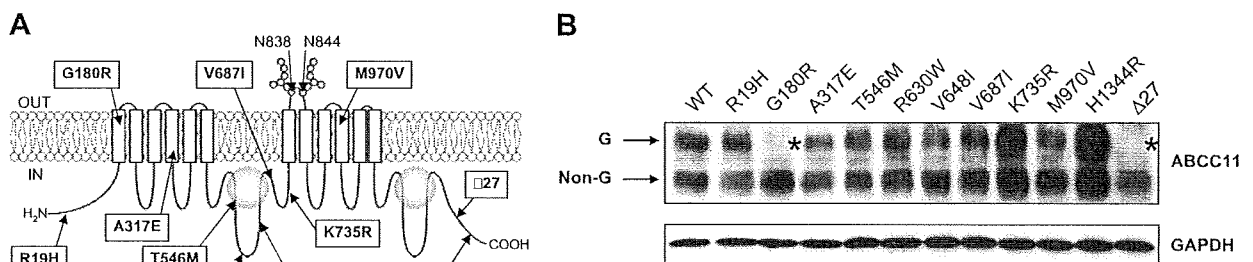
Figure 6. Effect of nonsynonymous SNPs and a \Delta 27 mutation on the N -linked glycosylation status of ABCC11. A ) Locations of hitherto reported nonsynonymous SNPs and \Delta 27 are indicated in putative structure of ABCC11. B ) Variants of nonsynonymous SNPs and \Delta 27 were created by site-directed mutagenesis with PCR primers listed in Supplemental Table 3. Those variant forms were expressed in Flp-In-293 cells. N -linked glycosylated (G) and nonglycosylated (non-G) forms of ABCC11 protein were detected by immunoblotting. Asterisk (*) indicates no N -linked glycosylation of ABCC11. C ) Levels of ABCC11 WT and \Delta 27 mutant proteins in Flp-In-293 cells. Samples were processed in the same manner as described in Fig. 4A. D ) Effect of MG132 on expression levels of ABCC11 WT and \Delta 27 mutant proteins. ABCC11 and GAPDH (loading marker) were detected by immunoblotting. Data are expressed as means \pm SD; n = 3 .
