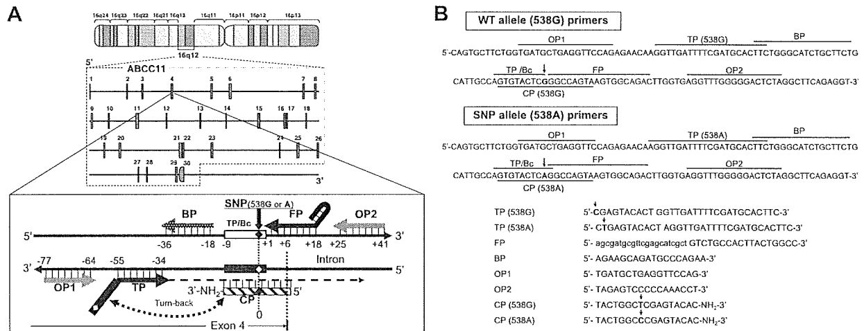
Figure 7. Strategy for SmartAmp-based detection of SNP 538G>A in ABCC11 gene. A) Schematic illustration of SmartAmp-based SNP detection. SNP 538G>A resides in exon 4 of ABCC11 gene on chromosome 16q12. B) Partial genomic DNA sequences of ABCC11 gene carrying WT (538G) and SNP (538A) alleles and sequences of primers used for SmartAmp assay.
