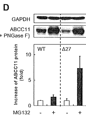
Figure 6. Effect of nonsynonymous SNPs and a \Delta 27 mutation on the N -linked glycosylation status of ABCC11. A ) Locations of hitherto reported nonsynonymous SNPs and \Delta 27 are indicated in putative structure of ABCC11. B ) Variants of nonsynonymous SNPs and \Delta 27 were created by site-directed mutagenesis with PCR primers listed in Supplemental Table 3. Those variant forms were expressed in Flp-In-293 cells. N -linked glycosylated (G) and nonglycosylated (non-G) forms of ABCC11 protein were detected by immunoblotting. Asterisk (*) indicates no N -linked glycosylation of ABCC11. C ) Levels of ABCC11 WT and \Delta 27 mutant proteins in Flp-In-293 cells. Samples were processed in the same manner as described in Fig. 4A. D ) Effect of MG132 on expression levels of ABCC11 WT and \Delta 27 mutant proteins. ABCC11 and GAPDH (loading marker) were detected by immunoblotting. Data are expressed as means \pm SD; n = 3 .
