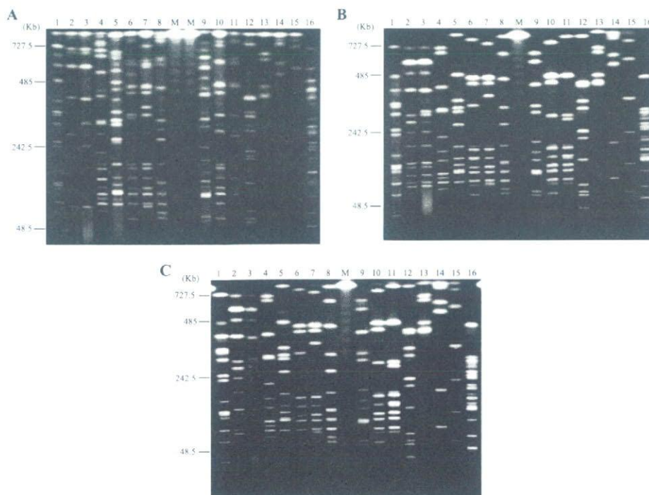
Fig. 2. PFGE profiles obtained with the conventional (A) and improved (B and C) protocols for Legionella strains. Lambda ladder marker (Bio-Rad) was used as a DNA size standard and molecular sizes are indicated on the left. Lane 1, 80-045; lane 2, K6; lane 3, Philadelphia-1; lane 4, NIIB0733; lane 5, NIIB0805; lane 6, NIIB0744; lane 7, NIIB0802; lane 8, NIIB0784; lane 9, NIIB0792; lane 10, NIIB0794; lane 11, NIIB0806; lane 12, NIIB0008; lane 13, NIIB0009; lane 14, NIIB0010; lane 15, NIIB0012; lane 16, NIIB0052; M: lambda ladder marker. A white smeary band at the bottom of the gel A (e.g., in lanes 3, 5, 9, and 10) indicates DNA damage.
