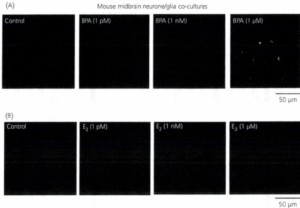
FIG. 7. A high concentration of bisphenol-A (BPA), but not 17 \beta -oestradiol ( E_2 ), causes a neuronal cell death in mouse midbrain neurone/glia cocultures. Mouse midbrain neurone/glia cocultures were incubated with normal medium, BPA (1 pM, 1 nM or 1 \mu M; A) or E_2 (1 pM, 1 nM or 1 \mu M; B) for 24 h. All cells were stained with a polyclonal antibody to cleaved caspase-3.
