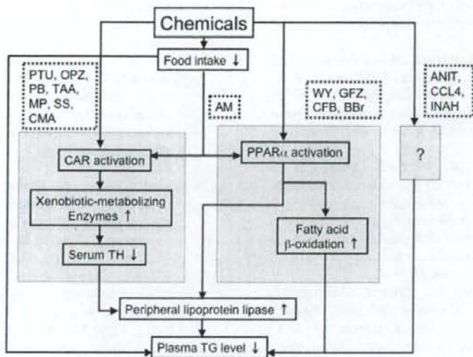
Fig. 4. Proposed TG-decreasing mechanisms of various drugs elucidated by comprehensive gene expression analysis.
