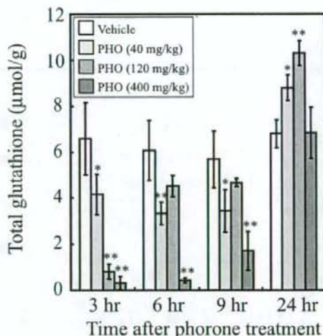
Fig. 2. Hepatic glutathione content after phorone treatment.
