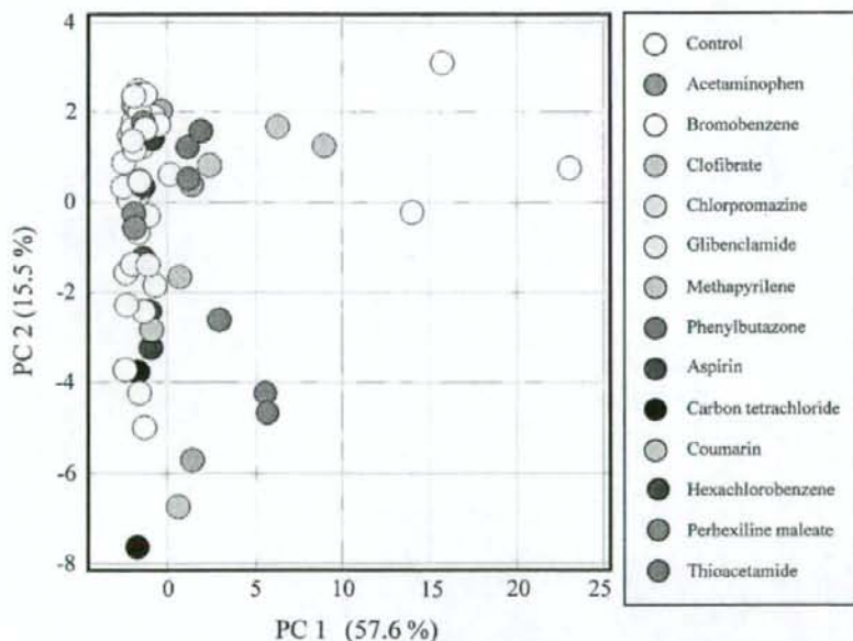
Fig. 4. PCA for GeneChip data of rat liver 24 hr after treatment with various hepatotoxicants. PCA was performed using GSH probe sets for GeneChip data of rat livers 24 hr after treatment with various hepatotoxicants. Each spot, colored by chemical type, represents individual samples. Bromobenzene, coumarin, and acetaminophen showed apparent shift from control, suggesting a perturbation of glutathione homeostasis in the liver after treatment.
