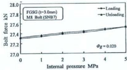
Fig. 8 Behavior of bolt force in flange joint subjected to internal pressure (using flexible graphite gasket).
