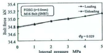
Fig. 6 Behavior of bolt force in flange joint subjected to internal pressure (using flexible graphite gasket).
