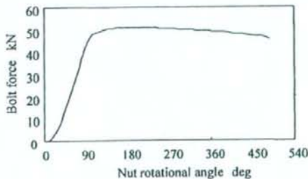
(b) Relation between axial bolt force and nut rotational angle
