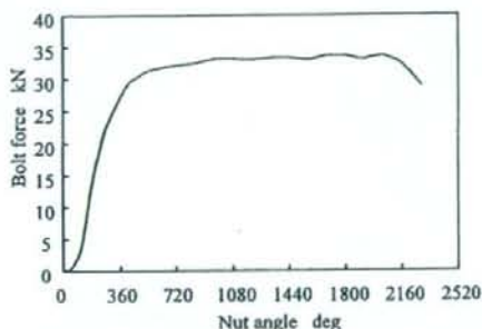
Fig. 1 Relation between axial bolt force and nut angle (using M8 bolt).
