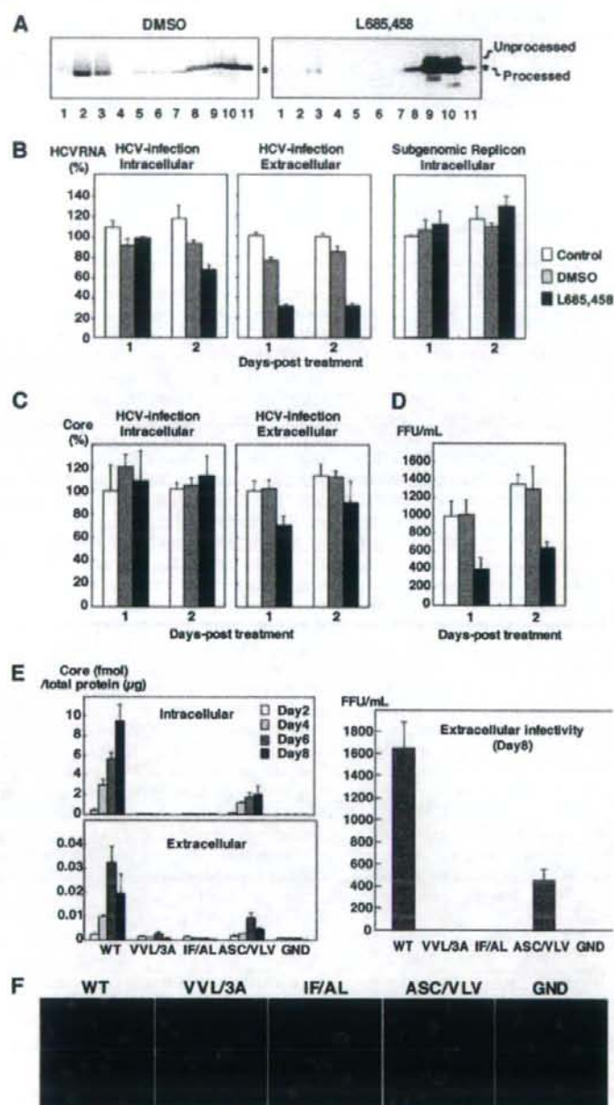
FIG. 6. Effect of the processing of HCV core protein by SPP on the propagation of JFH-1 virus. (A) L685,458 was added, at a concentration of 25 \mu\text{M} , to the culture supernatant of Huh7OK1 cells persistently infected with HCV strain JFH-1. Cells harvested at 24 h after treatment were lysed with 1% Triton X-100 and subjected to a flotation assay. DRM (lanes 1 to 7) and detergent-soluble (lanes 8 to 11) fractions were identified based on the localization of the marker proteins (data not shown). Asterisks indicate processed core proteins. DMSO, dimethyl sulfoxide. (B to D) Cells persistently infected with HCV strain JFH-1 were harvested at 1 or 2 days after treatment with the inhibitor. The data shown in each panel are representative of three independent experiments. (B) Total RNA was prepared from the cells (left) and the culture supernatant (center). Levels of HCV viral RNA and GAPDH mRNA were determined by real-time quantitative PCR. Values for the levels of viral DNA were normalized to that for GAPDH mRNA as described in Materials and Methods. The subgenomic-replicon cell line 9-13 was treated with the inhibitor, and total
