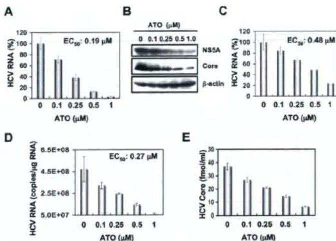
FIG. 1. Inhibition of HCV replication by ATO. (A) The level of genome-length HCV RNA in O cells after the treatment with ATO was monitored by real-time LightCycler PCR. Experiments were done in triplicate and, bars represent the mean percentage of HCV RNA. Error bars indicate standard deviations. (B) HCV core and NS5A protein expression levels in O cells after treatment with ATO. The results of Western blot analysis of cellular lysates with anti-HCV core, anti-HCV NS5A, or anti- \beta -actin antibody in O cells at 72 h after treatment with ATO at the indicated concentration are shown. (C) The level of subgenomic replicon RNA was monitored by real-time LightCycler PCR. Results from three independent experiments conducted as described for panel A are shown. (D) The level of intracellular genome-length HCV-JFH1 RNA was monitored by real-time LightCycler PCR. RSc cells were pretreated with the indicated concentration of ATO for 13 h, followed by inoculation of the HCV-JFH1 virus, and then the infected cells were further incubated with ATO for 97 h. Results from three independent experiments conducted as described for panel A are shown. (E) The levels of the core protein in the culture supernatants treated as described for panel D were determined by enzyme-linked immunosorbent assay. Experiments were done in triplicate, and bars represent the mean core protein levels.
