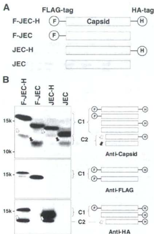
FIG. 2. The C2 protein lacks the amino terminus. (A) Series of the capsid protein constructs with or without FLAG and HA tags in the amino and carboxyl termini, respectively. (B) Expression of a series of the capsid proteins in Vero cells. The cell lysates expressing F-JEC-H, F-JEC, JEC-H, and JEC were examined by immunoblotting using anti-capsid, anti-FLAG, and anti-HA antibodies. The molecules detected by the immunoblotting are indicated on the right. White and black arrows indicate the C2 proteins with and without HA tags in the carboxyl terminus, respectively.
