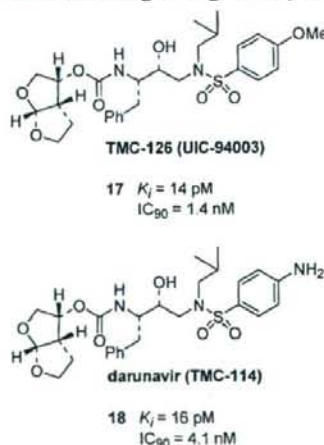
FIGURE 4. Bis-THF-Derived Protease Inhibitors.
