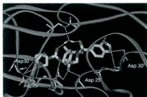
FIGURE 6. Crystal structure of Inhibitor 21-bound HIV-1 protease.
