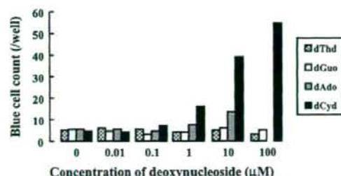
Fig. 3. Reversal of the antiviral activity of EFdA in the presence of 2-deoxynucleosides. Each 2-deoxynucleoside was added to the medium with serial dilution in the presence of EFdA (3.5 nM). The effect on EFdA activity was determined by the MAGI assay. An ADA inhibitor, dCF, was used during dA competition.
