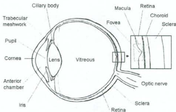
Figure 31-2. Schematic diagram of the human eye.
