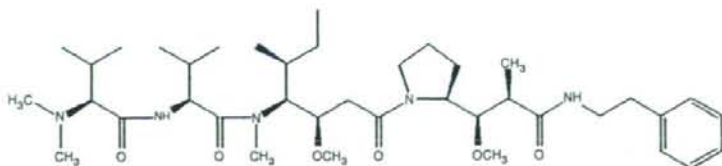
Figure 1 Chemical structure of TZT-1027.
