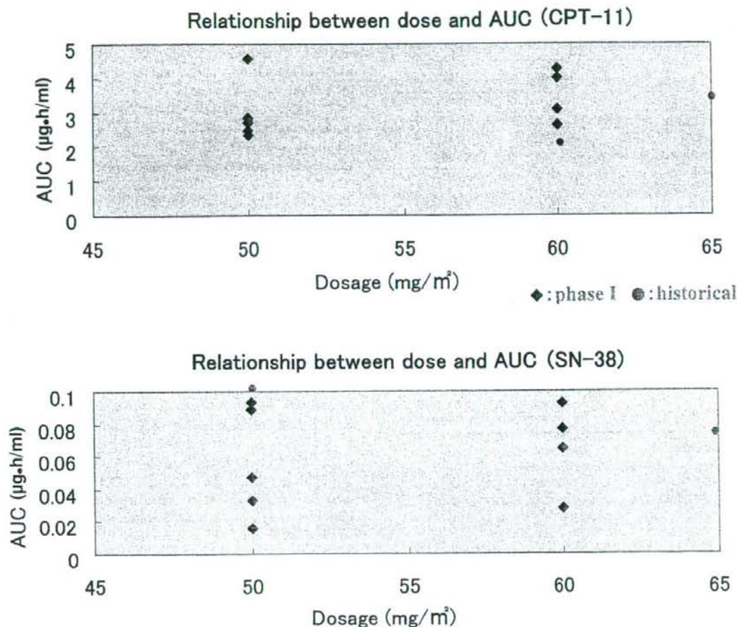
Figure 2. Relationship between dose ( \text{mg}/\text{m}^2 ) and area under the concentration-time curve (AUC) ( \mu\text{g}\cdot\text{h}/\text{ml} ) of (A) irinotecan; (B) SN-38.
