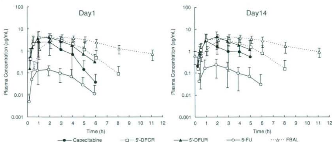
Figure 3. Plasma concentrations (mean \pm standard deviation) for capecitabine and its metabolites 5'-deoxy-5-fluorocytidine (5'-DFCR), 5'-deoxy-5-fluorouridine (5'-DFUR) and \alpha -fluoro- \beta -alanine (FBAL).
