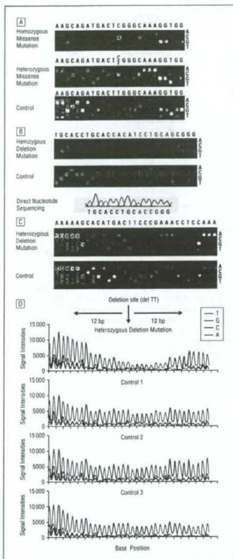
Figure 3. Validation of accuracy of sequence determination. A, Scan images of homozygous and heterozygous SOD1 L126S mutations. Each column shows a base position, and each row shows a base call (the determination of base(s) at each position). In the center position, the base call was T in the control, whereas in the patients, the base calls were homozygous C (upper panel) or heterozygous C/T (middle panel). B, Scan image of hemizygous ABCD1 del2146-2157 mutation. Signals of the deletion site and surrounding probes were virtually undetectable. C, Scan image of heterozygous SOD1 L129 (del459TT) mutation. The base calls at the mutation site of the patient were the same as those of the control. The probes at and around the mutation site, however, showed decreased signal intensities compared with those of the controls. D, Signal intensities at and around the deletion site of heterozygous SOD1 L129 (del459TT) mutation. Signal intensities at the deletion site (del TT) and the flanking bases were approximately half those of the controls. bp indicates base pairs.
