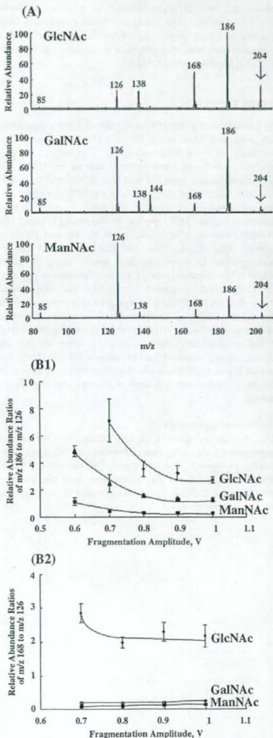
Figure 7. (A) Positive ion ESI-MS 3 spectra of GlcNAc, GalNAc and ManNAc generated from precursor ion [M-H_2O+H]^+ at m/z 204. Fragmentation amplitude is 0.8 V. The precursor ion is indicated with a vertical arrow. The relative abundance ratios of (B1) m/z 186 to 126 and (B2) m/z 168 to 126 in MS 3 spectra at the different fragmentation amplitudes for GlcNAc, GalNAc, and ManNAc. The fragment ion at m/z 186 was detected above 0.5 V for ManNAc, and 0.6 V for GlcNAc and GalNAc. The fragment ion at m/z 168 was detected above 0.6 V for GlcNAc, and 0.7 V for GalNAc and ManNAc. The fragment ion at m/z 126 was detected above 0.6 V for GalNAc and ManNAc, and 0.7 V for GlcNAc.
