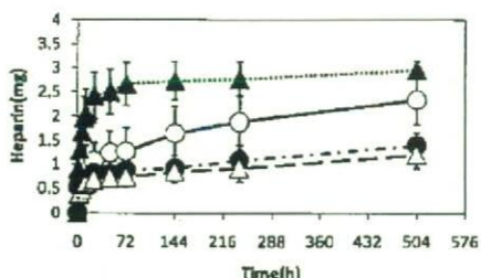
Fig. 1. Cumulative release of heparin from PVA hydrogel.
