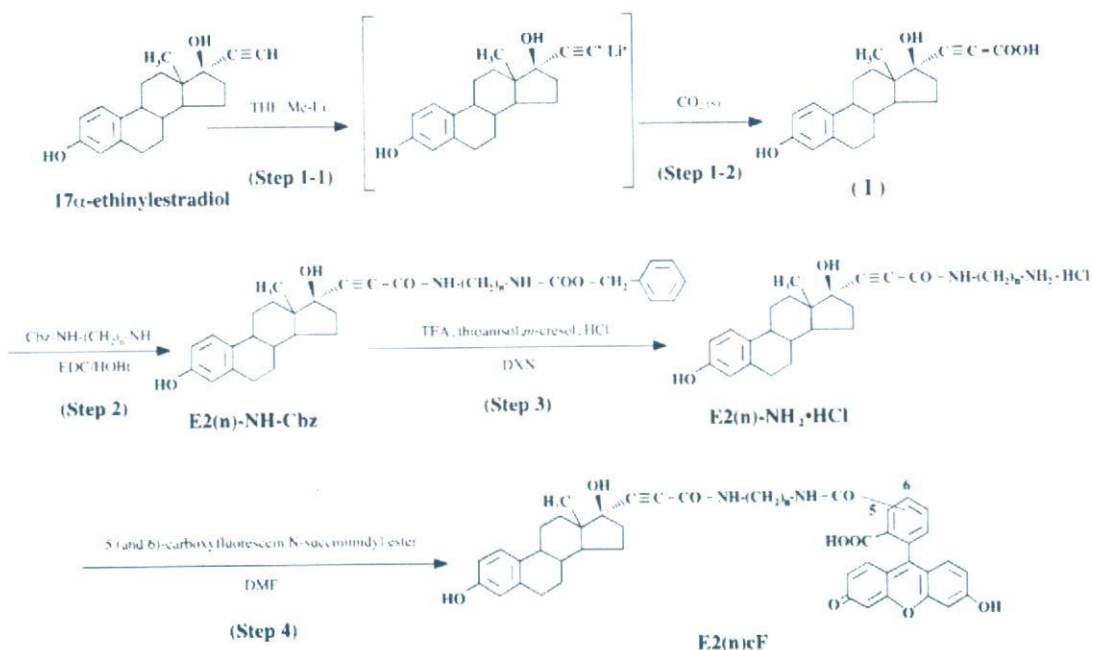
Fig. 1. Synthetic scheme of the conjugates of 17 \alpha -ethinylestradiol and carboxyfluorescein via \alpha,\omega -diamino alkanes \text{H}_2\text{N}-(\text{CH}_2)_n-\text{NH}_2 ( n=2, 4, 6, 8, 10 and 12 ).
