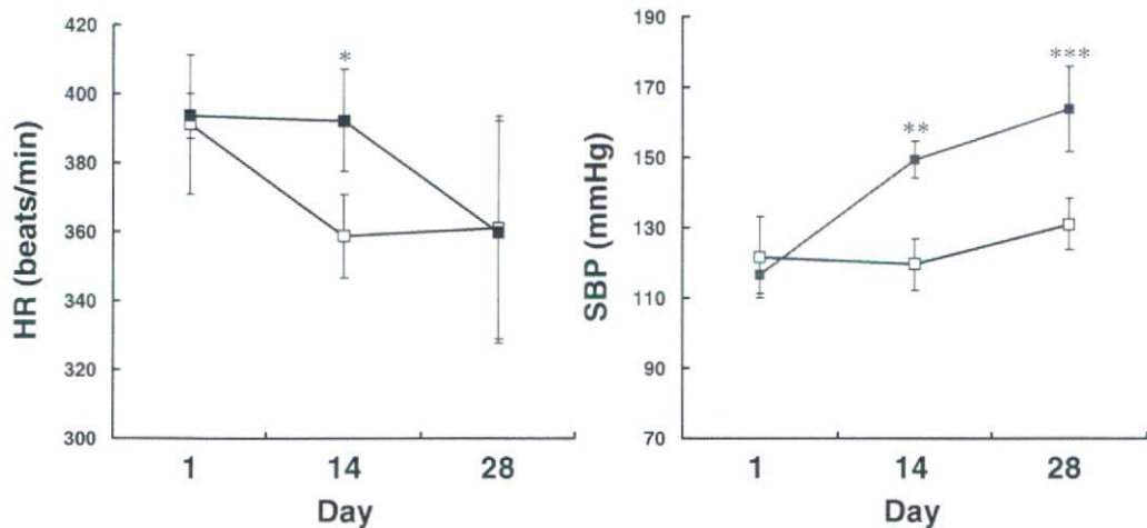
Fig 3. Effect of whole-body inhalation exposure of carbon black (CB) on heart rate (HR) and blood pressure (BP), which were measured by tail-cuff plethysmography after 1, 14, and 28 days of exposure. Each point represents a group of 3 rats. (Open squares) Control group (n=3), (filled squares) CB-treated group (n=3). Although HR measured on days 1 and 28 did not differ between the control and CB groups, HR on day 14 was significantly elevated in the CB group compared with the control group. In rats exposed to CB, levels of systolic BP (SBP) increased in an exposure-time dependent manner. Asterisks denote significant differences between the groups: * p=0.0383 , ** p=0.0046 , and *** p=0.0164 . Vertical bars indicate standard deviation.
