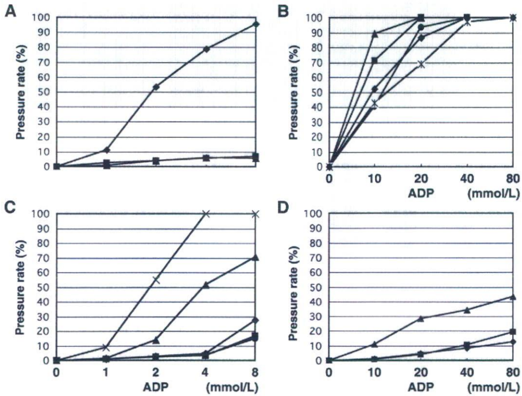
Fig 7. Platelet aggregation, as analyzed by screen filtration pressure method in carbon black (CB) or water-soluble fullerene (C 60 (OH) 24 )-treated whole blood. (A) Concentration response curve of platelet aggregation to adenosine diphosphate (ADP) (◆; 0, 10, 20, 40, 80 mmol/L), CB (▲; 0, 50, 100, 200 μg/ml) and C 60 (OH) 24 (■; 0, 5, 10, 25, 50 μg/ml). (B) High-concentration ADP (●; 0, 10, 20, 40, 80 mmol/L), CB (*; 50 μg/ml, ◆; 100 μg/ml), C 60 (OH) 24 (■; 25 μg/ml, ▲; 50 μg/ml), and (C) low-concentration ADP (◆; 0, 1, 2, 4, 8 mmol/L). ADP-induced aggregation was facilitated by C 60 (OH) 24 (■; 2.5 μg/ml, ▲; 25 μg/ml, ×; 50 μg/ml) in a dose-dependent manner, but CB (*; 50 μg/ml, ●; 100 μg/ml) had no effect. (D) High-concentration ADP (0, 10, 20, 40, 80 mmol/L), C 60 (OH) 24 (■; 2.5 μg/ml, ▲; 10 μg/ml) upregulated platelet aggregation, despite inhibition by ticlopidine hydrochloride (◆; 2 mmol/L).
