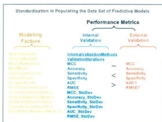
Figure 1. MAQC-II data analysis: Generating a large data set of predictive models for meta-analysis
