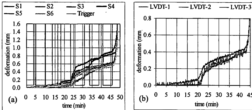
Figure 7. Deformation for Slope-V-2 (a) Slope surface and (b) Slope top
