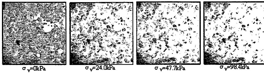
Figure 11. The change in the CLSM image of NSF-clay as the increase in the normal stress (170μm×170μm).
