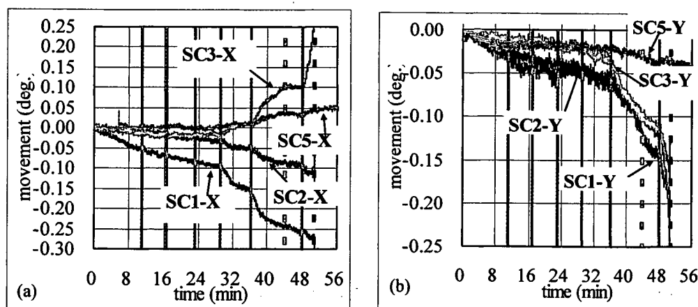
Figure 11. SA type tilt sensor measurement for Narita sand model (a) X and (b) Y directions
