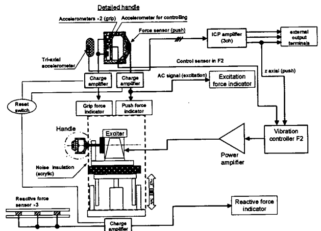
Fig. 2 Schematic diagram of New JIS T8114 based vibration transmissibility measurement system.
