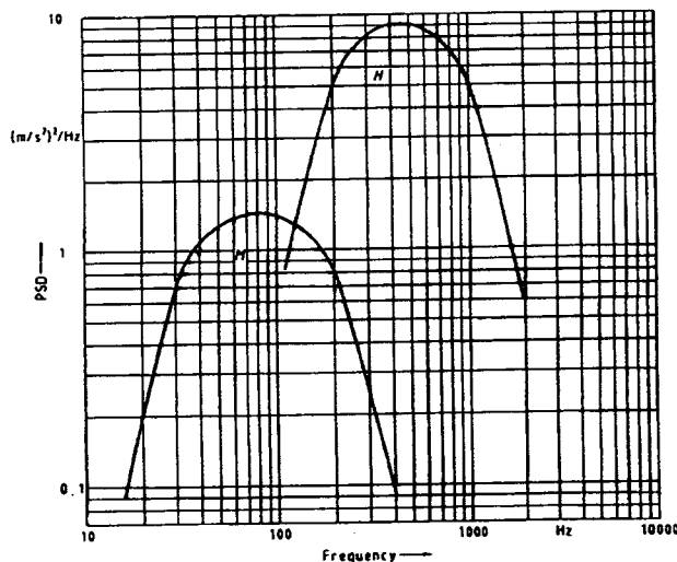
Fig. 1 Spectra of the two vibration signals (M and H).
