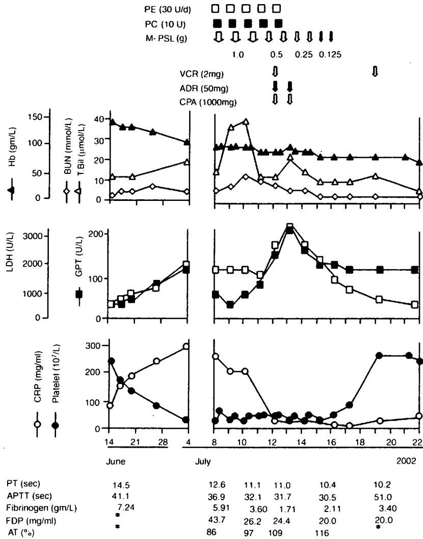
Figure 2. Time course of laboratory parameters and therapeutic regimen. PE, plasma exchange; PC, platelet concentration; m-psi, methyl prednisolone; VCR, vincristine; ADR, adriamycin; CPA, cyclophosphamide; Hb, hemoglobin; BUN, blood urea nitrogen; T.Bil, total bilirubin; LDH, lactate dehydrogenase; GPT, glutamic-pyruvic transaminase; CRP, C-reactive protein; PT, prothrombin time; APTT, activated partial thromboplastin time; FDP; fibrinogen degradation products; AT, antithrombin.
