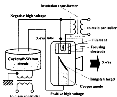
Fig. 18. Circuit diagram of the microfocus x-ray generator.
