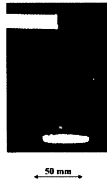
Fig. 8. Radiogram of water falling into a polypropylene beaker from a glass test tube.
