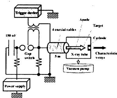
Fig. 9. Block diagram of the high-intensity super-fluorescent plasma flash x-ray generator
