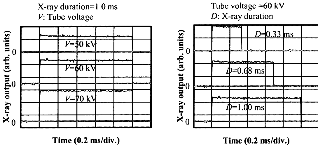
Fig. 2. X-ray outputs at indicated conditions.
