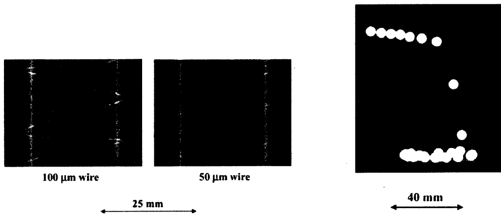
Fig. 4. Radiogram of plastic bullets falling into a polypropylene beaker from a plastic test tube.
