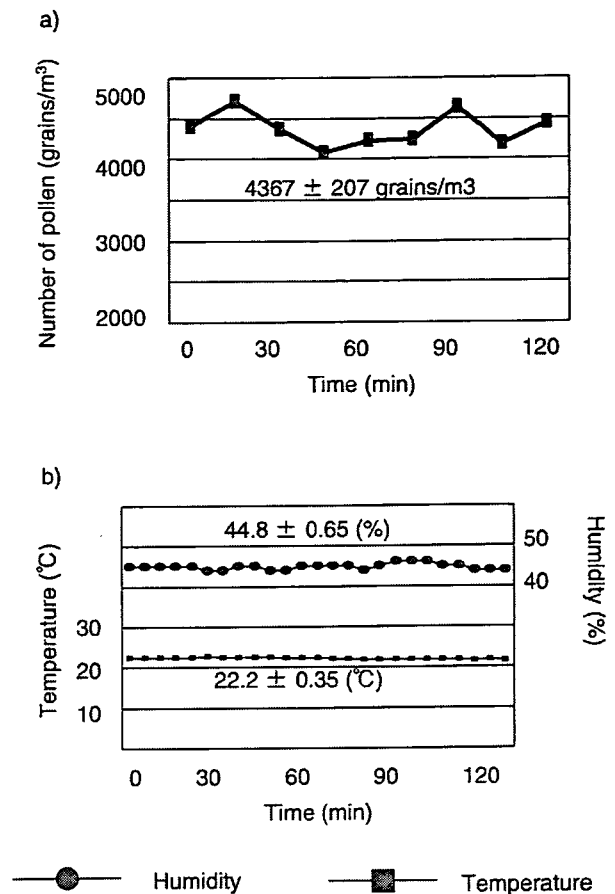
Fig. 5 The pollen count (a) and temperature and humidity (b) in the chamber during the second part of the study. The average number of pollen grains was 4367 ± 207 grains/m 3 , the average temperature 22.2 ± 0.35°C, and the average humidity 44.8 ± 0.65%.
