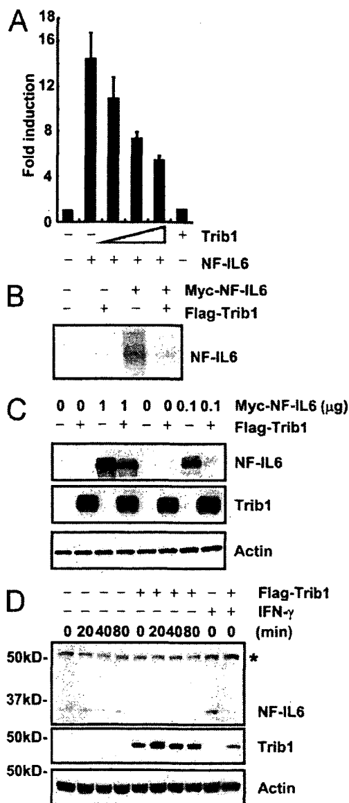
Figure 3. Inhibition of NF-IL6 activity by Trib1 overexpression.
