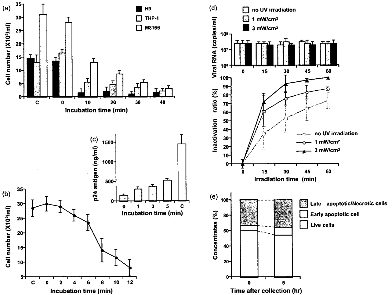
Fig. 1. Cytotoxicity of breast milk and a modified cell-free virus-associated infection assay. (a) Evaluation of cytotoxicity of breast milk to several cell lines (C, untreated control); (b) detailed course of cytotoxicity to M8166 cells within a 12-min period; (c) a modified cell-free virus-associated infection assay using a shorter exposure time and higher virus concentration than the conventional assay (C, conventional assay control). Alteration of infectious viral particles and BMCs in breast milk; (d) alteration of infectious viral particles in breast milk and comparison with the viral copies quantified from viral RNA by PCR. All the data shown are mean \pm S.D. from three independent experiments performed in triplicate; (e) evaluation of BMC viability in breast milk by flow-cytometric analysis. The data shown are means, and are representative of four separate experiments.
