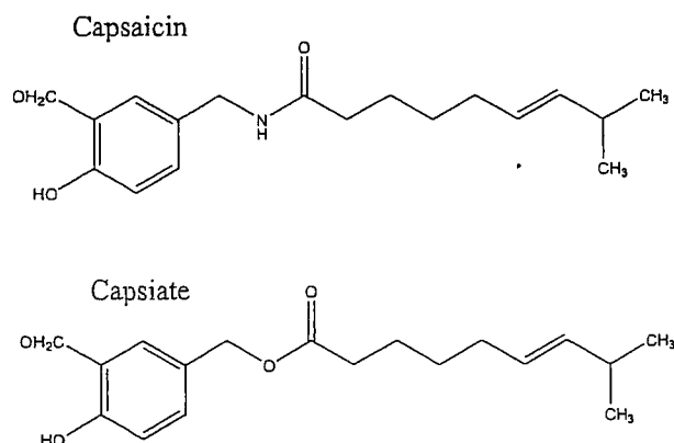
Figure 1 Structures of capsaicin and capsiate.
