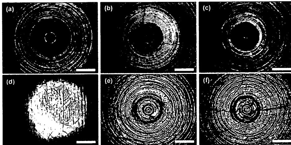
Figure 6. Confocal laser scanning microscope images of the CLPE and CLPE- g -MPC bearing surfaces before and after the hip simulator test. (a) CLPE (gamma-ray sterilized), (b) CLPE- g -MPC (nonsterilized), (c) CLPE- g -MPC (gamma-ray sterilized) before the hip simulator test, (d) CLPE (gamma-ray sterilized), (e) CLPE- g -MPC (nonsterilized), and (f) CLPE- g -MPC (gamma-ray sterilized) after the hip simulator test. The bar indicates 500 \mu\text{m} .
