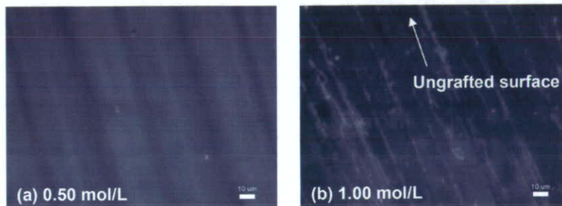
Figure 6. FM images of CLPE-g-MPC obtained with various MPC concentrations and a 90-min photo-irradiation time. Bar; 10 μm. [Color figure can be viewed in the online issue, which is available at www.interscience.wiley.com.]
