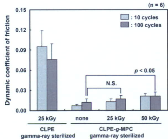
Figure 4. Dynamic coefficients of friction of gamma-ray sterilized CLPE surfaces and nonsterilized and gamma-ray sterilized CLPE-g-MPC surfaces. Bar, Standard deviations.
