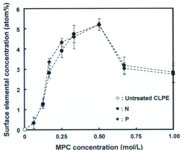
Figure 2. Surface elemental concentration of CLPE-g-MPC as a function of the MPC concentration with a 90-min photo-irradiation time.
